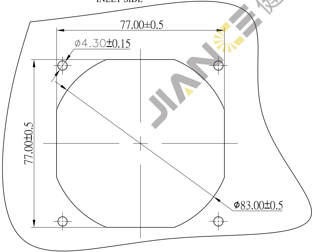
INLET SIDE
