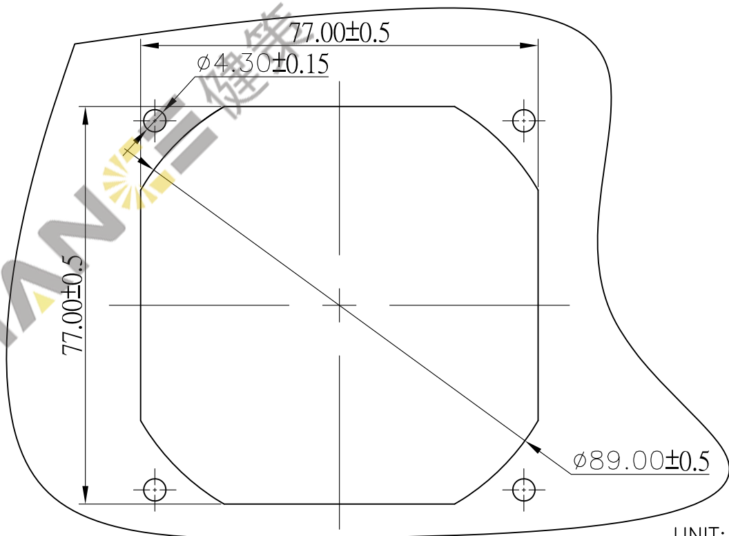
OUTLET SIDE
